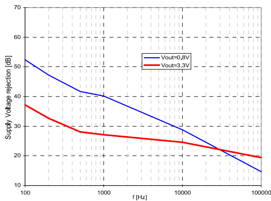
Figure 10: Supply voltage rejection vs frequency
