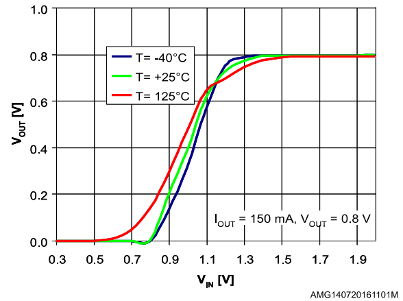
Figure 5: Output voltage vs input voltage ( V_{OUT} = 0.8 \text{ V} )
