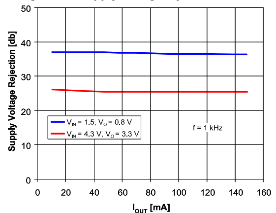
Figure 11: Supply voltage rejection vs IOUT
