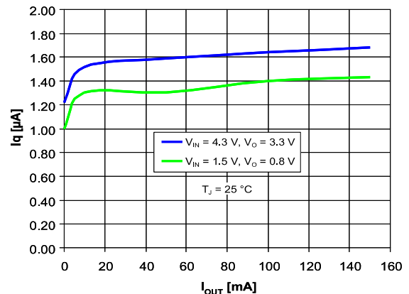
Figure 13: Quiescent current vs output current
